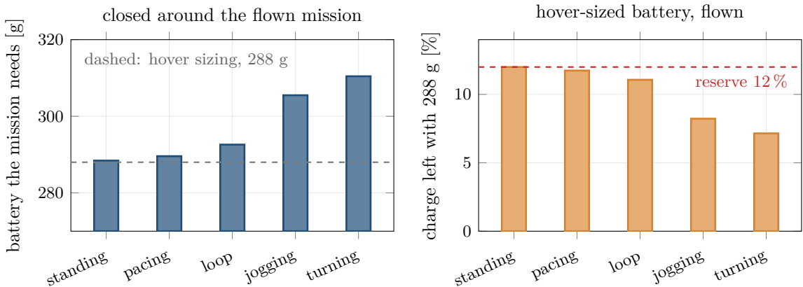
Figure 66: The coupled closure against the hover sizing. Left: the battery each motion needs when eq. (139) is solved around the flown mission; the dashed line is the 288 g of the hover sizing. Right: the charge left at t_f when that hover-sized pack is flown through each motion instead. Every moving mission lands below the 12 % reserve. The two panels are the same fact from either side: the right is the violation, the left is its cure.
