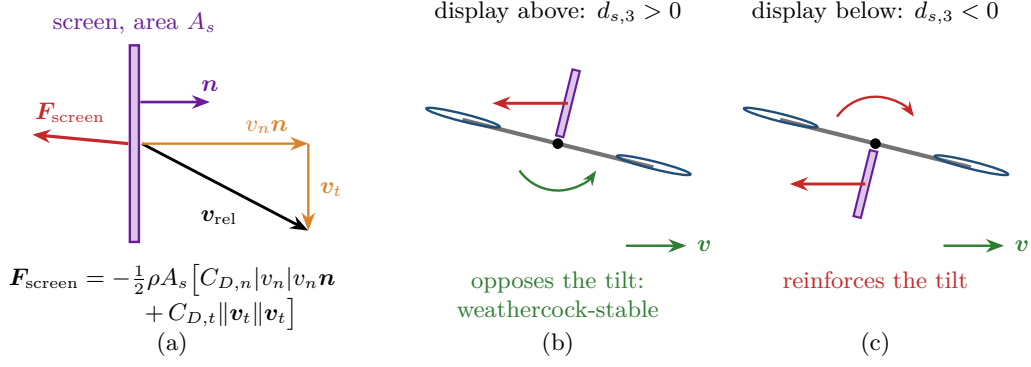
Figure 37: (a) The flat-plate model eq. (99). The plate’s velocity relative to the air splits into a normal part v_n\mathbf{n} , resisted with C_{D,n} over the whole area, and a tangential part \mathbf{v}_t , resisted only by skin friction, so the drag points almost along -\mathbf{n} whatever the direction of motion. (b), (c) The moment of that drag about the centre of mass in forward flight, airframe tilted toward the motion. With the display above, the moment turns the airframe back against its tilt; with the display below, further into it. The magnitude is the same; the sign is not.
