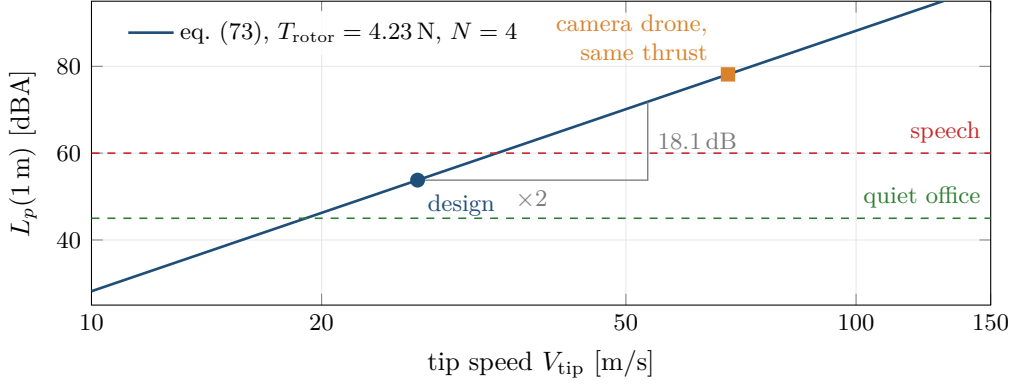
Figure 27: The source model eq. (73) at the design’s thrust per rotor. On a logarithmic tip-speed axis the level is a straight line of 60 dB per decade, so halving the tip speed buys 18.1 dB wherever one starts. The design turns at 26.7 m/s; carrying the same thrust at a camera drone’s tip speed would cost about 24 dB, the difference between a quiet office and a raised voice.
