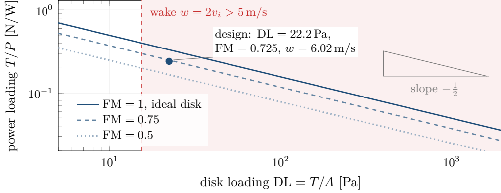
Figure 6: Power loading against disk loading, T/P = \text{FM}\sqrt{2\rho/\text{DL}} , from eq. (15) and the definition of FM in section 4. On logarithmic axes every figure of merit gives a line of slope -\frac{1}{2} : halving the disk loading buys a factor \sqrt{2} in thrust per watt, whatever the rotor. The shaded region is where the wake exceeds 5 m/s, the speed at which loose paper begins to move (requirement (R3) of section 17); the design sits just inside it, at \text{DL} = 22.2 \text{ Pa} and w = 6.0 \text{ m/s} .
