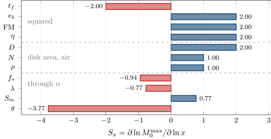
Figure 19: Logarithmic sensitivities of M_0^{\max} at the engine's default parameters, computed by central differences in ln-space. The top group are the squared levers of eq. (54); the middle group are disk area, entering as D^2 and N , and air density, eq. (55); the bottom group act through \alpha and are eq. (56), here with \gamma_m/\alpha = 0.257 . Every bar agrees with theorem 7.3 to three decimals. A bar of length two means a 10 % change in the parameter moves the critical load by about 20 %.
