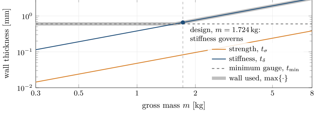
Figure 24: The three lower bounds of eq. (66) against gross mass for the design’s arm tube, r = 8.0 mm. Strength and stiffness are both linear in the limit load F \propto m , so on logarithmic axes they are parallel lines of slope one, and the stiffness bound lies a factor of about eight above the strength bound: an arm stiff enough is automatically strong enough. Below about 1.6 kg the minimum gauge governs; at the design, stiffness does.
