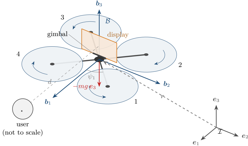
Figure 3: Frames and layout, to scale for the design of section 17 except for the user. \mathcal{I} is inertial with e_3 up; \mathcal{B} is attached at the centre of mass with b_1 along the screen normal toward the user, b_3 along the nominal thrust and b_2 = b_3 \times b_1 . The four rotors sit on arms at \psi_i = \pi/4 + (i-1)\pi/2 from b_1 (the \times layout) with alternating spin senses, marked by the arrows: rotors 1 and 3 turn anticlockwise seen from above, 2 and 4 clockwise. The display stands above the rotor plane, normal to b_1 , on a two-axis gimbal hinged at its lower edge. r locates the centre of mass in \mathcal{I} , and d is the standoff to the user's eye.
